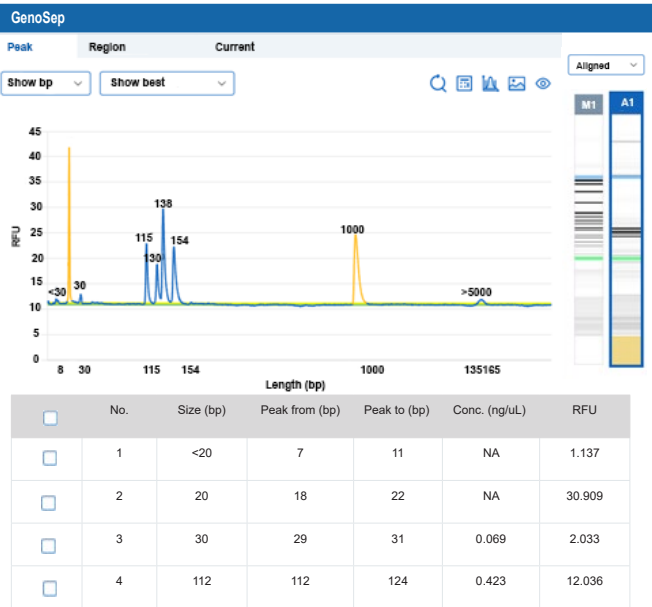
Figure 4: GenoSep software displays gel images, electropherograms, and fragment size data simultaneously.
