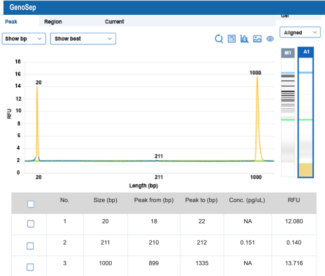
Figure 3: The LOD of the High Sensitivity DNA cartridge can reach down to 0.2 pg/μL.
