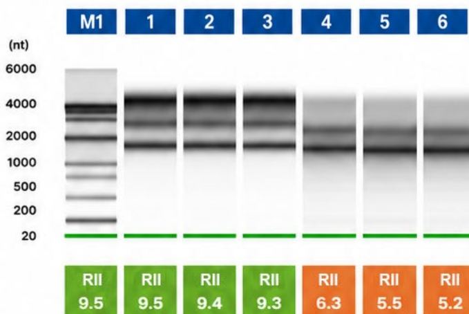
Figure 1: Fragmented HeLa RNA analysis on GenoSep. Lane M1: Marker. Lanes 1, 2 & 3: triplicate of HeLa RNA. Lanes 4, 5 & 6: triplicate run of processed HeLa RNA.
