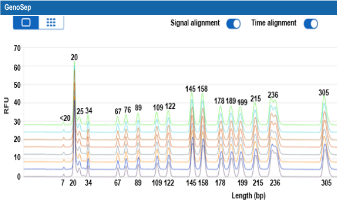
Figure 2: Repeated analysis of an identical marker sample demonstrates excellent fragment size accuracy and repeatability.
