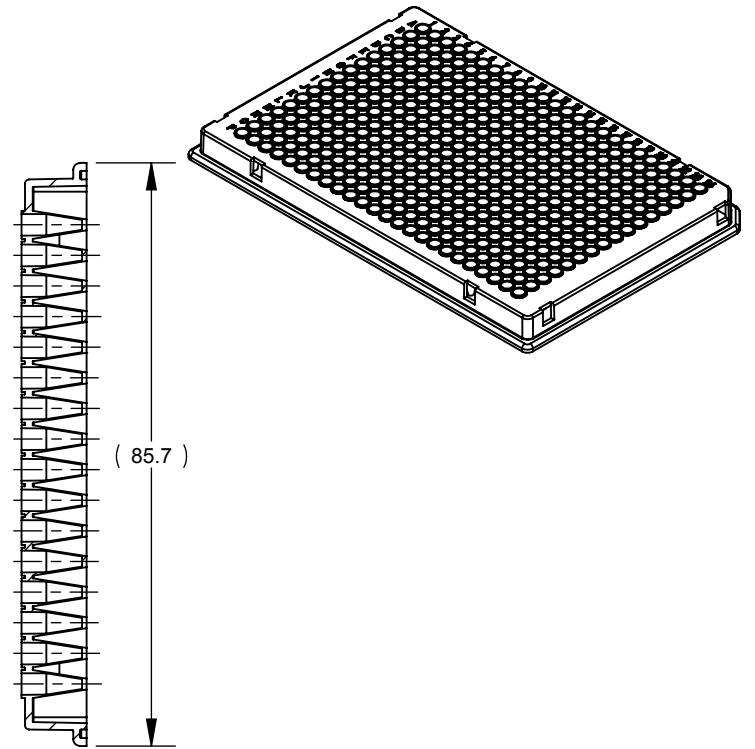
SECTION C-C
