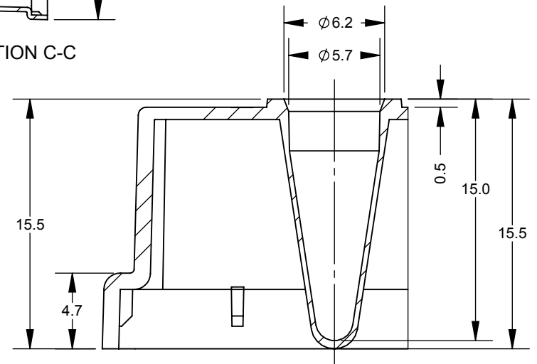
DETAIL B
