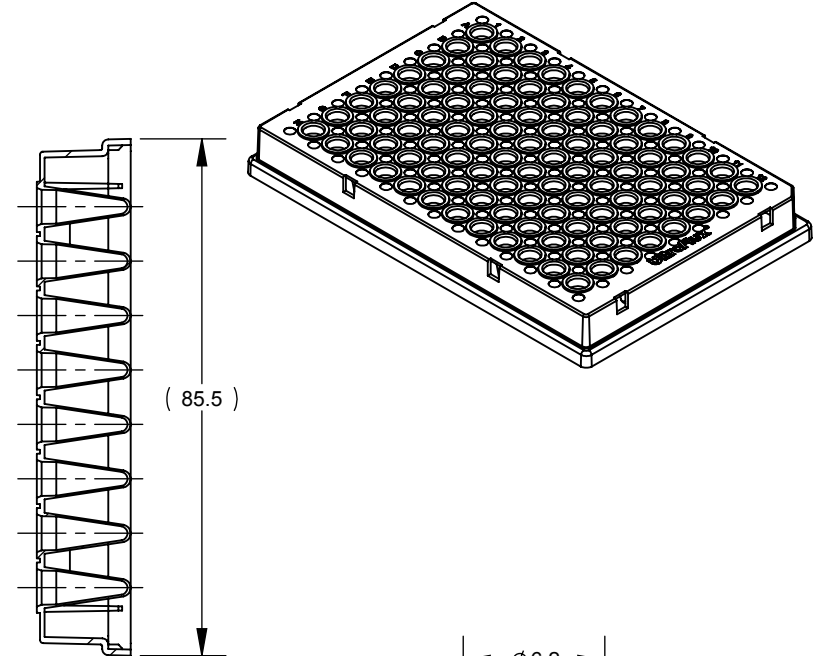
SECTION C-C
