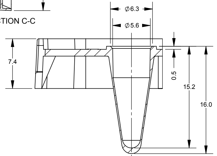
DETAIL B
